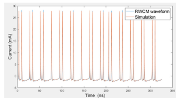
Figure 6: Chopped beam pattern measured after the SSR1 CM at 16.5 MeV. Minimum separation between bunches was 6.15 ns.
